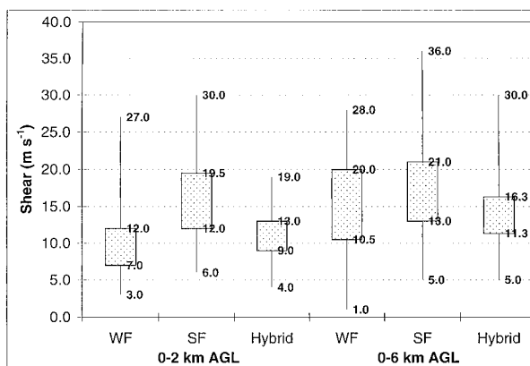
FIG. 5. As in Fig. 4 except for 0-2- and 0-6-km (all AGL) shear vector magnitudes with WF, SF, and hybrid events.
