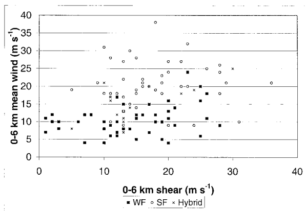
FIG. 16. As in Fig. 14 except for 0–6-km shear vs 0–6-km mean wind.
