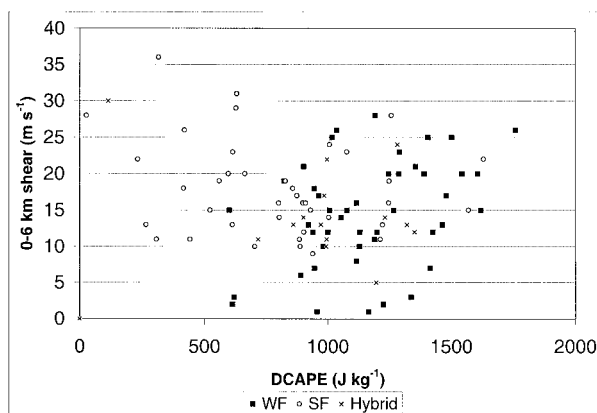
FIG. 15. As in Fig. 14 except for DCAPE vs 0–6-km shear.
