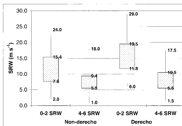
FIG. 22. As in Fig. 4 except for 0–2- and 4–6-km SRWs associated with WF nonderecho and derecho events.
