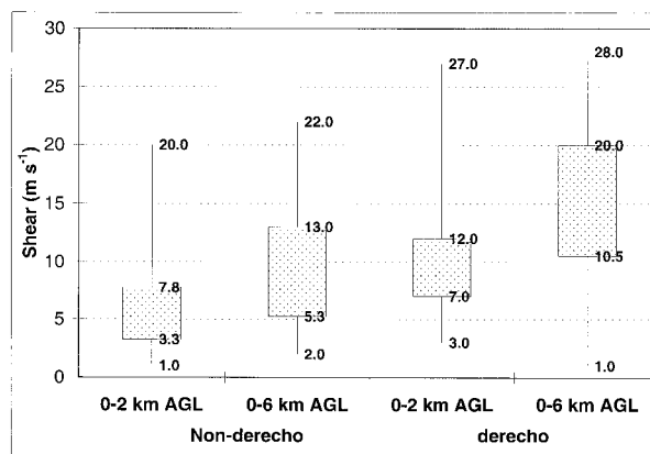
FIG. 21. As in Fig. 4 except for 0–2- and 0–6-km shear vectors for both nonderecho and derecho producing WF events.
