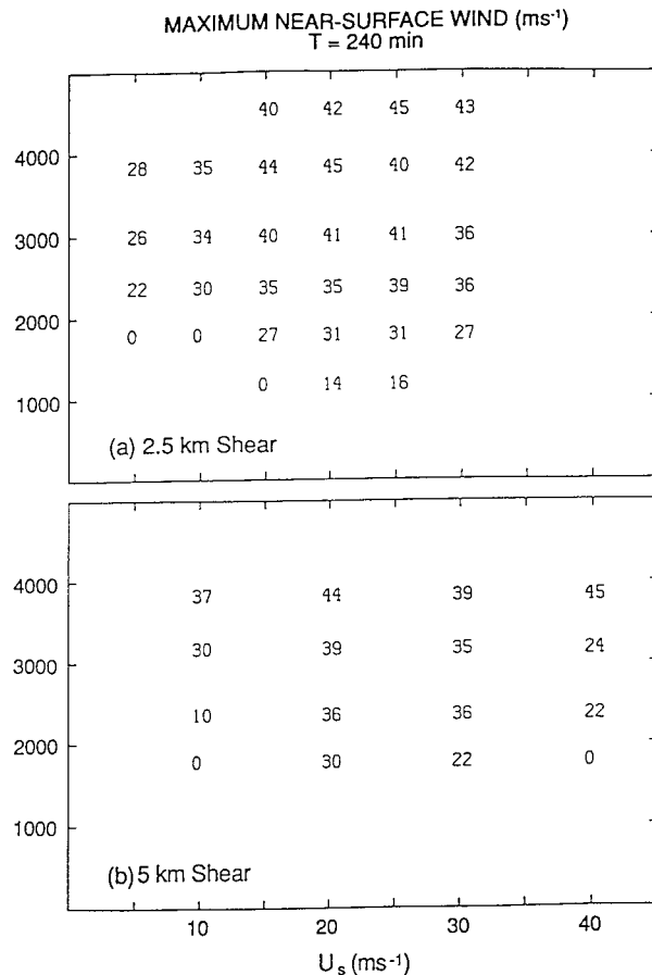
FIG. 23. Maximum near-surface (350 m) wind ( \text{m s}^{-1} ) for the (a) 2.5- and (b) 5-km shear from Weisman's numerical simulation (after Fig. 25 in Weisman 1993), plotted against corresponding CAPE used. Weisman considered severe surface winds to occur with 350-m winds of 35 \text{ m s}^{-1} . U_s represents the maximum magnitude of the wind for each wind profile.
