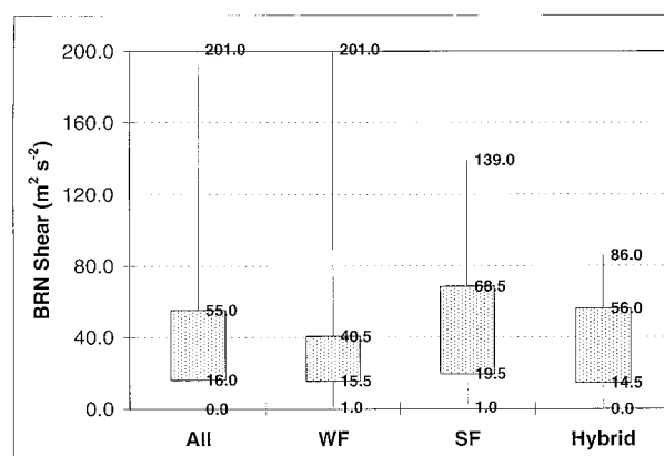
FIG. 8. As in Fig. 4 except for bulk Richardson number shear for all, WF, SF, and hybrid events.
