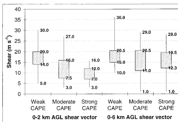
FIG. 13. As in Fig. 4 except for 0–2- and 0–6-km shear vector magnitudes distributed in varying MUCAPE environments. Weak, moderate, and strong categories represent MUCAPE classified by percentile rank in Fig. 9a (see text).
