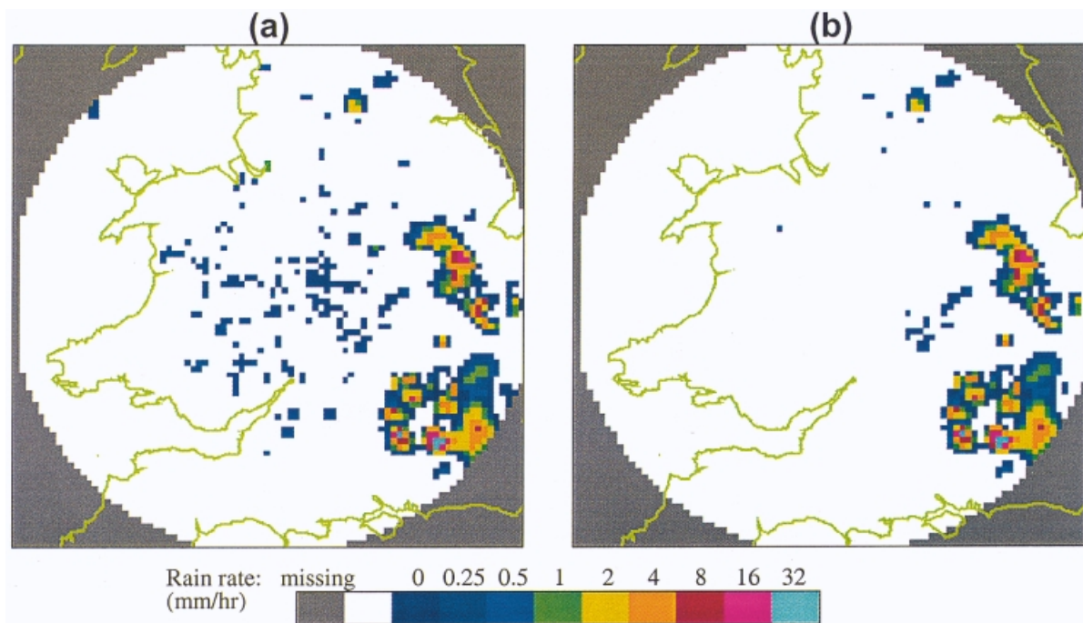
Figure 2. An example showing the removal of spurious echoes for a Clee Hill radar image: (a) the raw radar image and (b) the image after deletion of spurious echoes.
