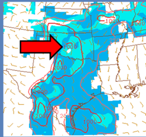
MLCAPE: 1000 j/kg
